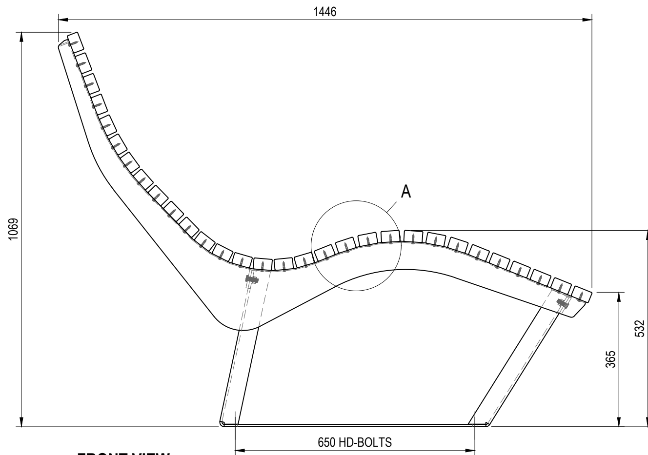
FRONT VIEW
