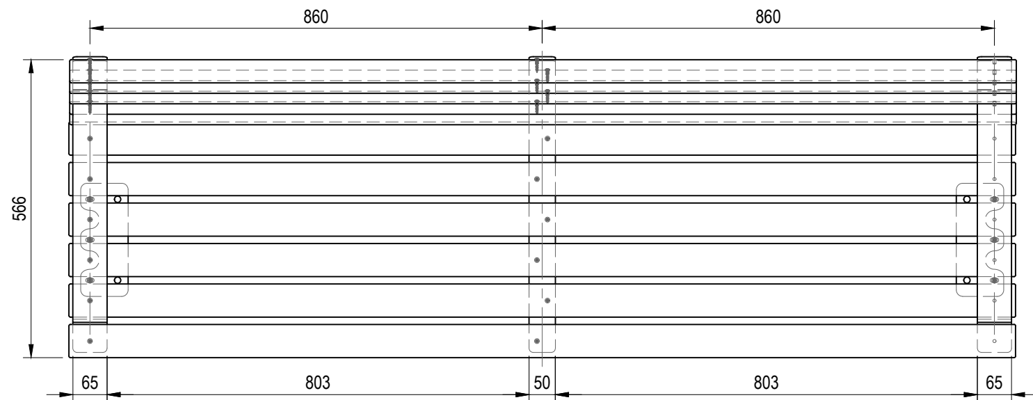
TOP VIEW
