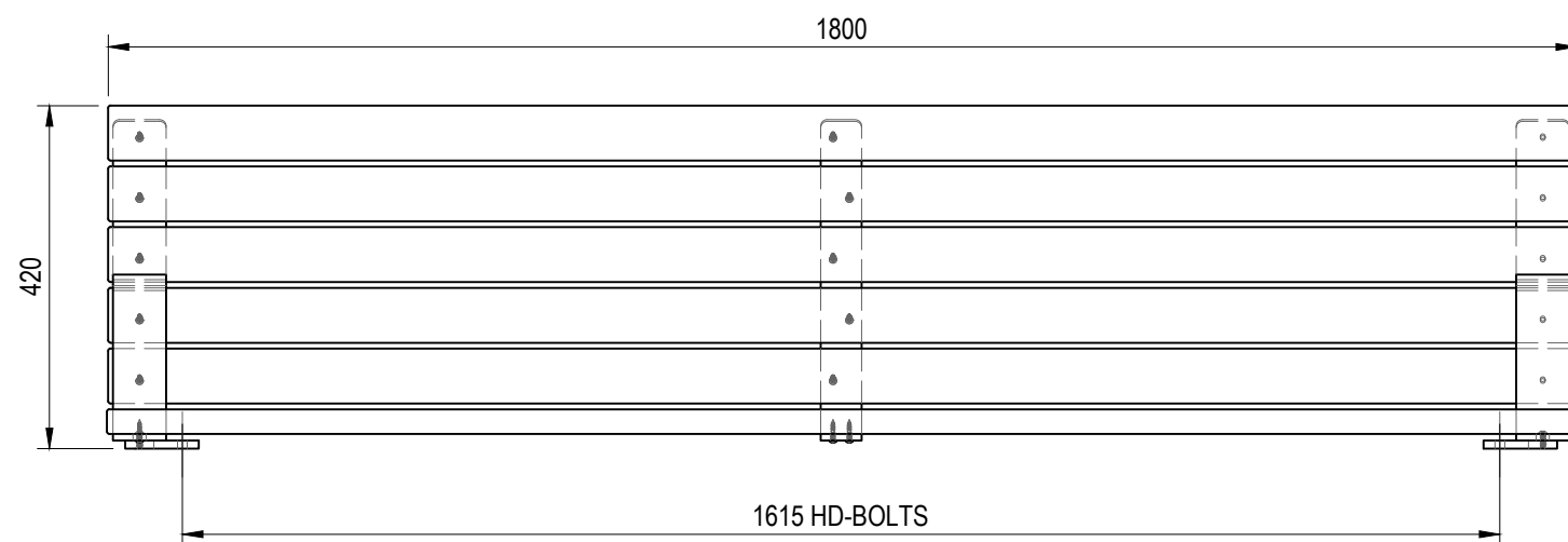
FRONT VIEW
