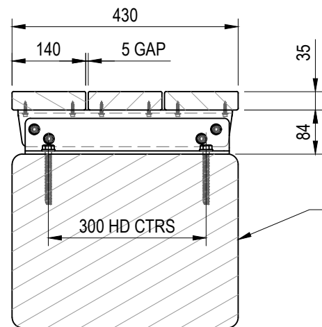
SECTION A-A (1:10)
