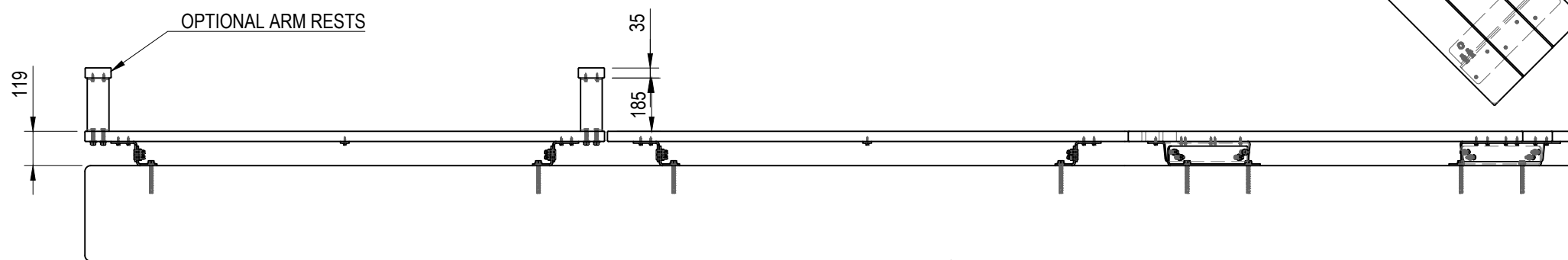
FRONT VIEW
