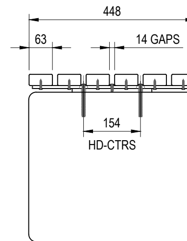
END VIEW
